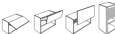
Flip-Up, Bi-Fold, Swing-Up, Tambour Door Cabinets sku ex: WP3018HK, HBPW3024HF, SUW3024HL, WTAM3042
