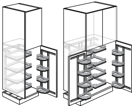
Tall Larder Cabinet
