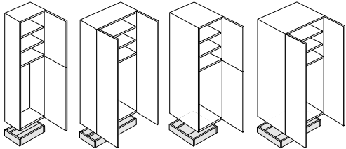
Classic Utility Cabinet
